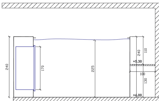
section 1-1
