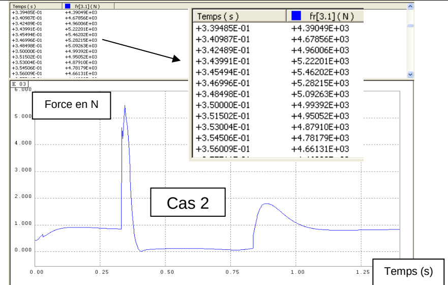
Effort roue/bras
