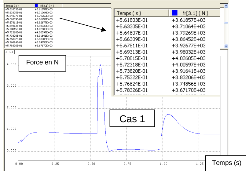
Effort roue/bras
